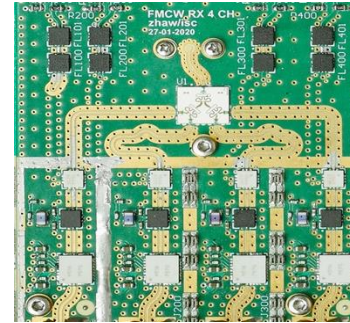
RF-Frontend
