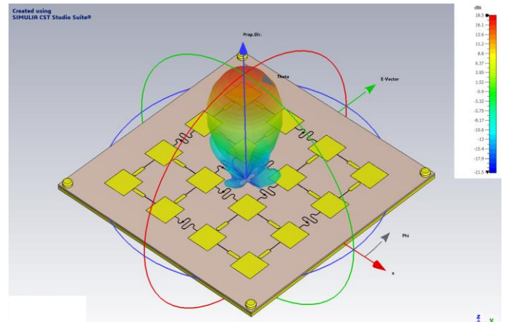
Antennensimulation (10 GHz)
