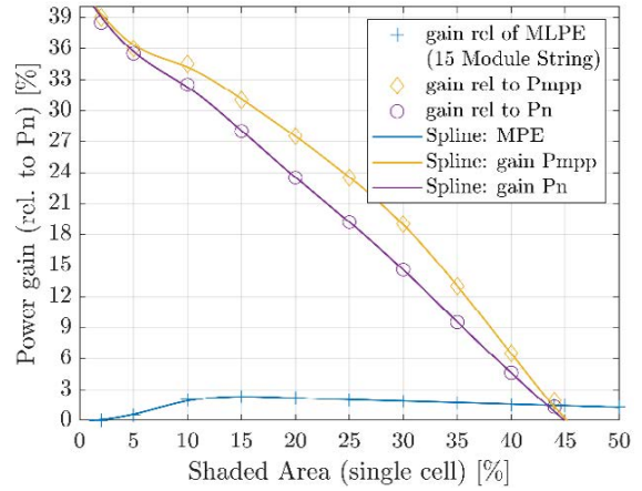
Figure 4: Plots and splines of the potential, relative MLPE system gains for shading of a single cell area in percent. Both, the module power gain relative to nominal module power (in violet) and the power gain relative to the power at the MPP (in yellow) are visualised. In blue, the relative total power gain of a MLPE system consisting of 15 modules in string.
