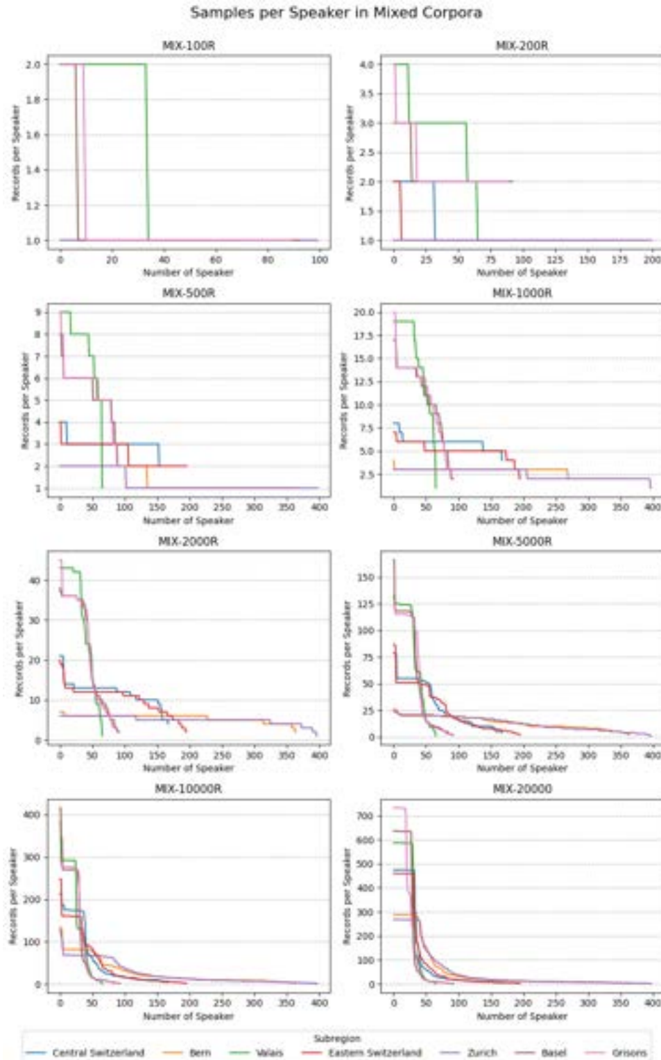
Figure 17: Samples per Speaker in Mixed Corpora
