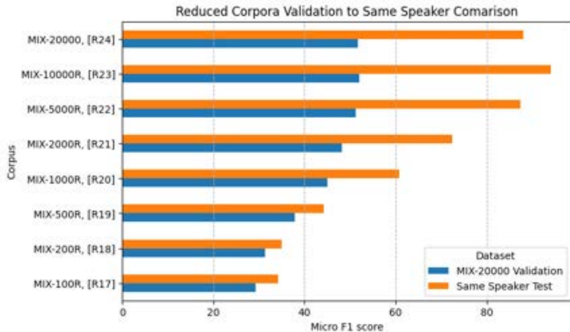
Figure 18: Reduced Corpora Validation to Same Speaker Comparison
