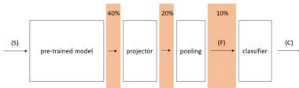
Figure 19: Drop Out Layers
