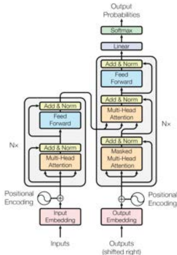
Figure 1: Transformer Architecture [38]
