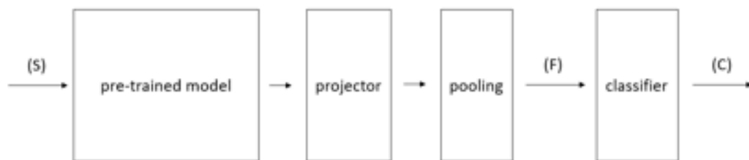
Figure 12: Model Architecture
