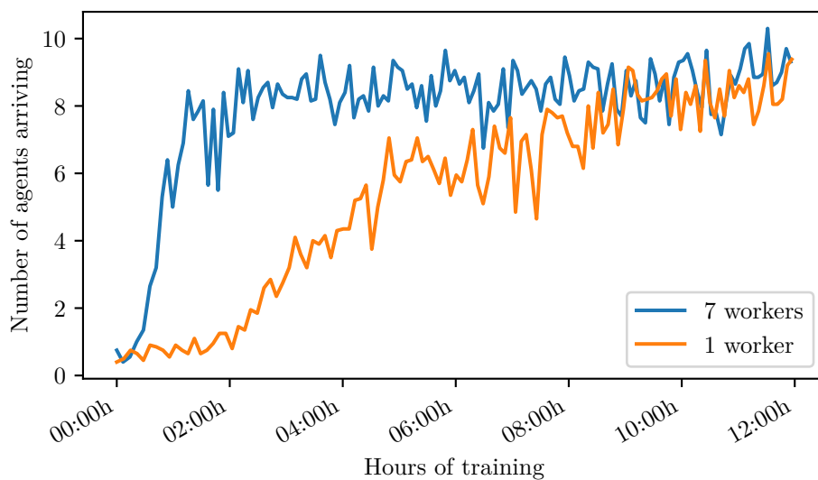
Figure 4.8: Comparison of training with 1 worker to training with 7 workers.
