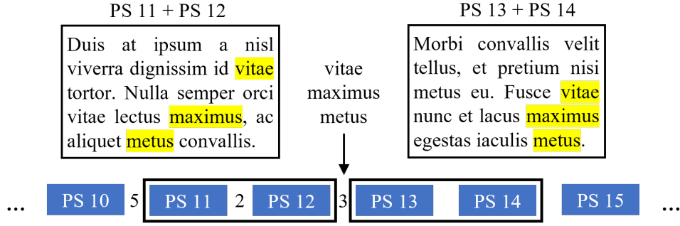
Figure 5: Block comparison method
