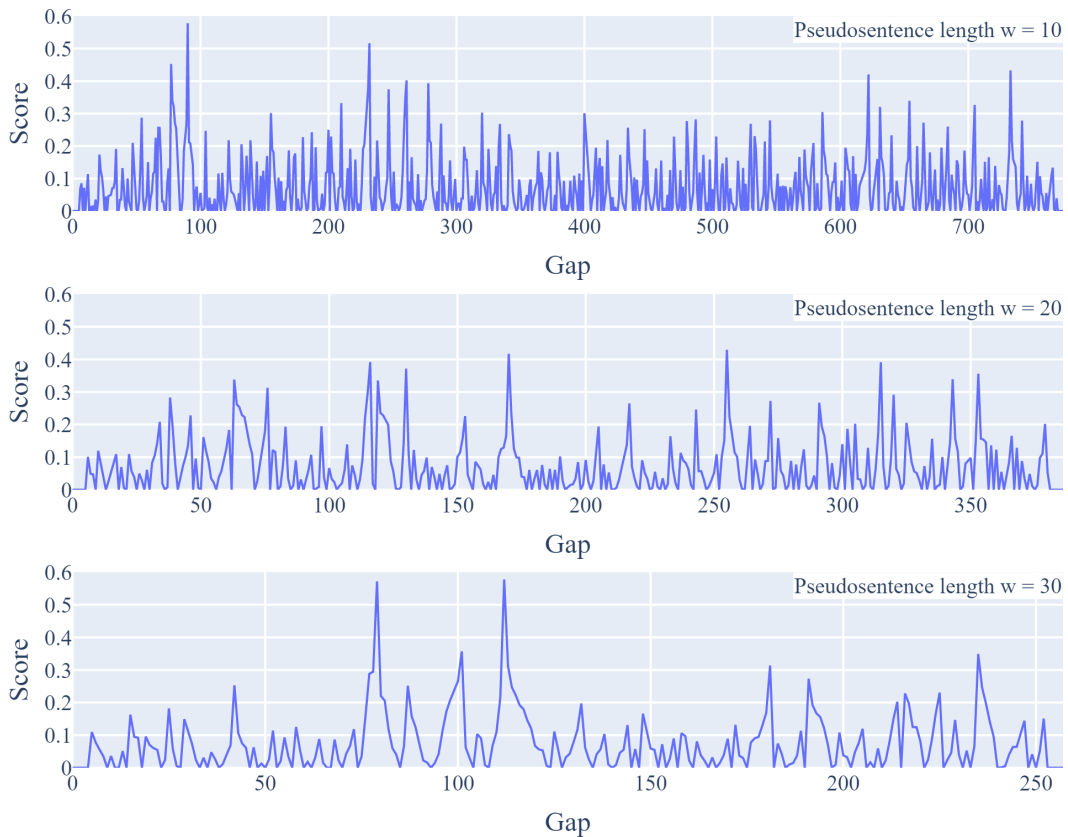
Figure 9: Depth scores of the vice presidential debate transcript with corresponding pseudosentence length
