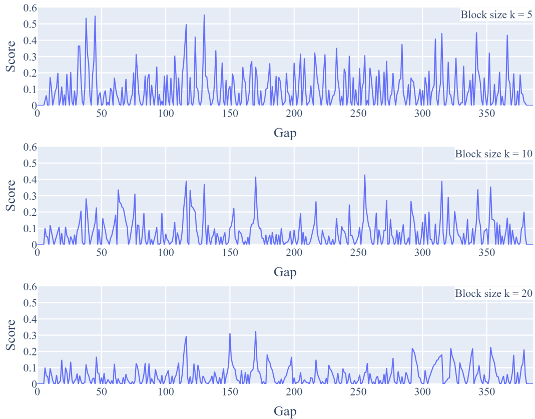
Figure 10: Depth scores of the vice presidential debate transcript with corresponding block size
